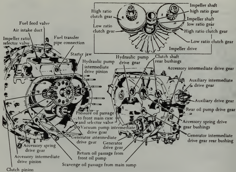
FIGURE 2-9. Intermediate rear and rear case sections.
